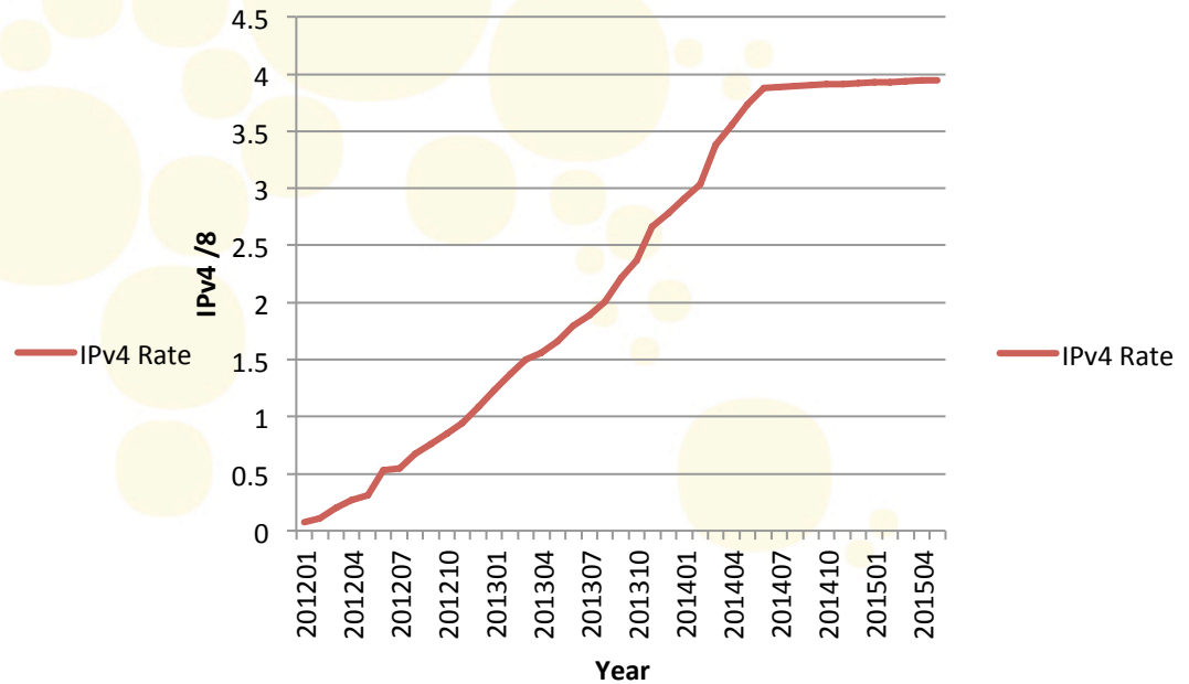
IPv4 /8 Accumulated
